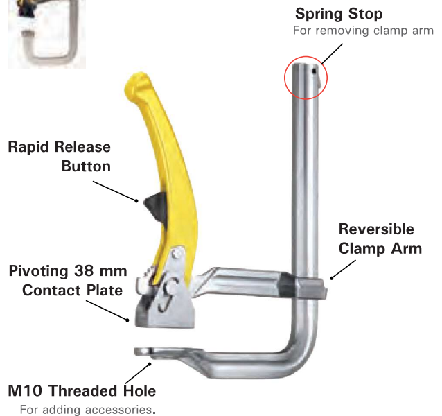
UF100JRM Sturdy J-shaped 76 mm return for step-over applications.
